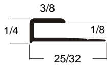
7820 BA 1/8" Cap 5', 8' or 10'
