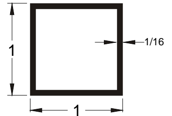
7360 S Square Tube 1" x 1" 6' or 12'
