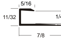
7830 BA 1/4" Coving Cap 8'
